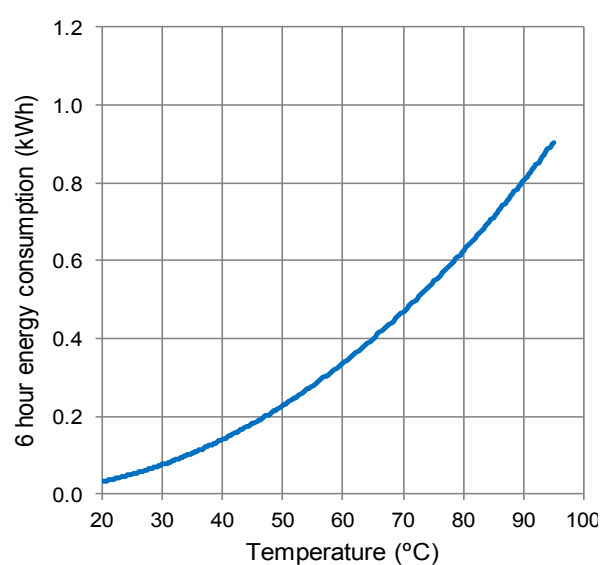
With lid
