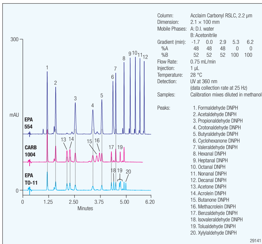
Figure 1. High-throughput analysis of DNPH aldehydes and ketones regulated by CARB 1004, EPA 554, and EPA TO-11 methods.
