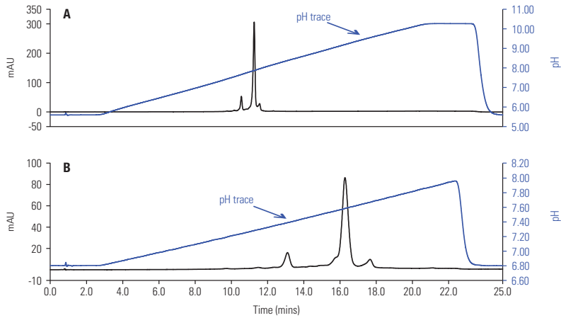
Figure 10: Faster separation of Monoclonal Antibody Variants using pH gradient on a MAbPac SCX-10 RS, 5 µm, 4.6 × 150 mm column
