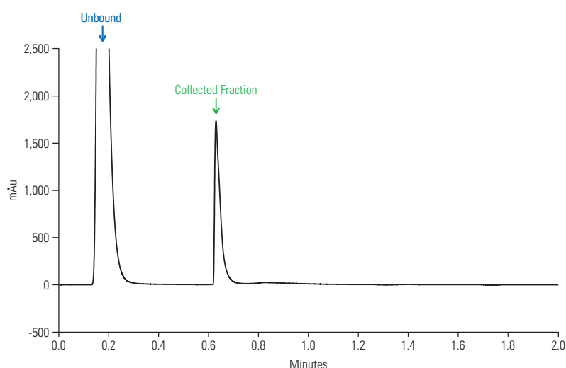
Figure 2: Purification of HCC on the MAbPac Protein A (4 × 35 mm) column
