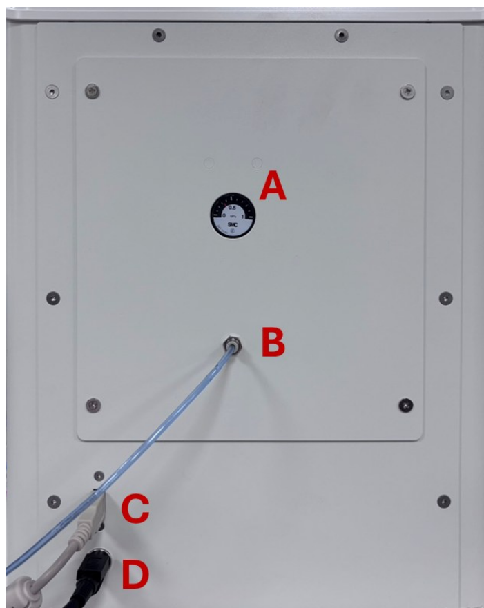
Figure 2 Back View of Qsep 100 2.0
