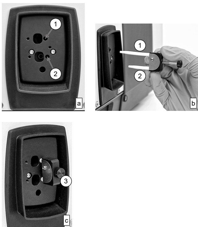
Fig. 6: Mounting the connection tube
