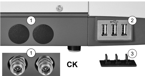
Fig. 3: Left side of the instrument
