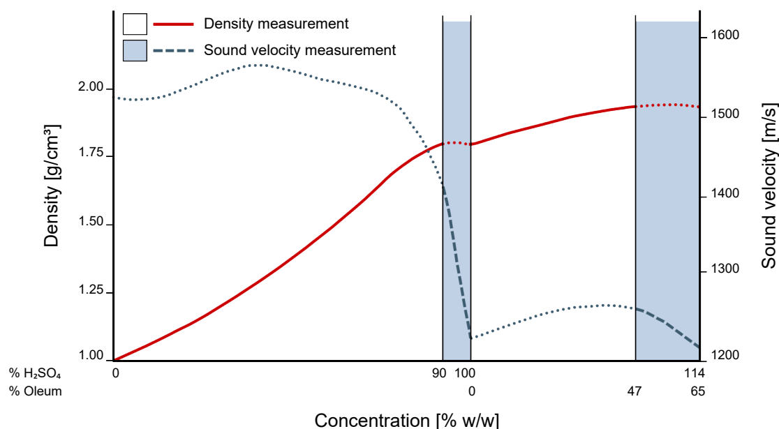
Fig. 25: Density and sound velocity of sulfuric acid and oleum at 40 °C
