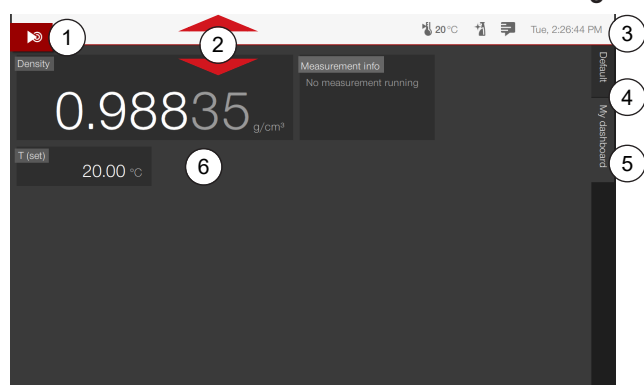
Fig. 22: Example dashboard
