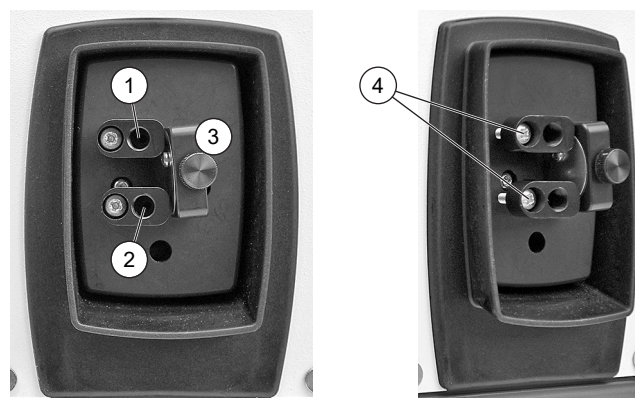
Fig. 7: Injection adapters and connection tube mounted
