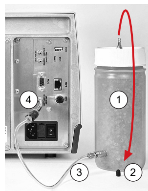
Fig. 24: Drying cartridge installed
