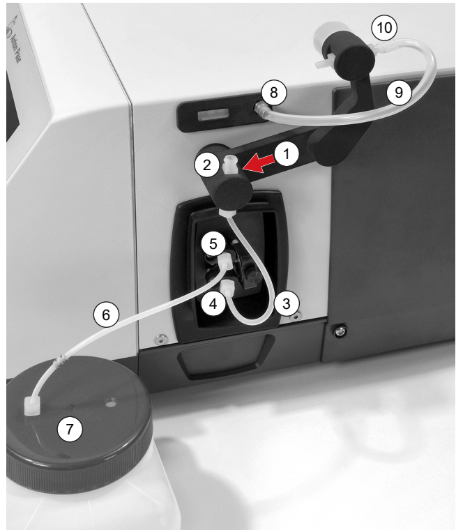
Fig. 8: Mounting U-Dry, all hoses, and waste vessel for standard measurements
