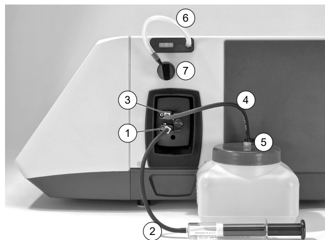
Fig. 10: All Viton hoses mounted
